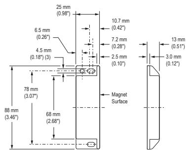
Figure 3. SI-MAG1MM/MM90/MMHF Magnet
