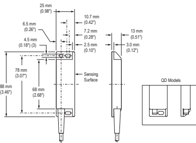
Figure 1. SI-MAG1SM Sensor
